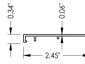
39 SIDELITE ADAPTER
