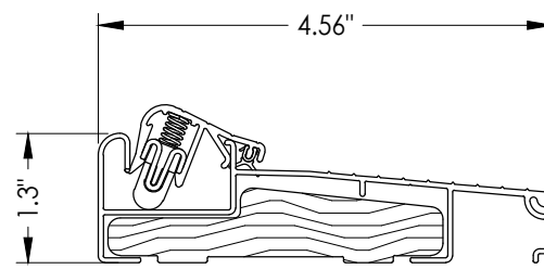
31 INSWING THRESHOLD Endura (Articulating) ALUM/WOOD
