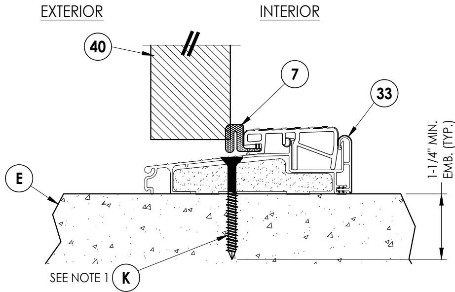
1 VERTICAL CROSS SECTION 8 Outswing configuration
