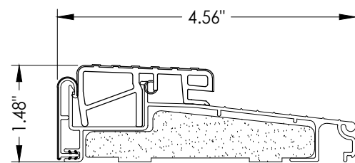
33 OUTSWING THRESHOLD
