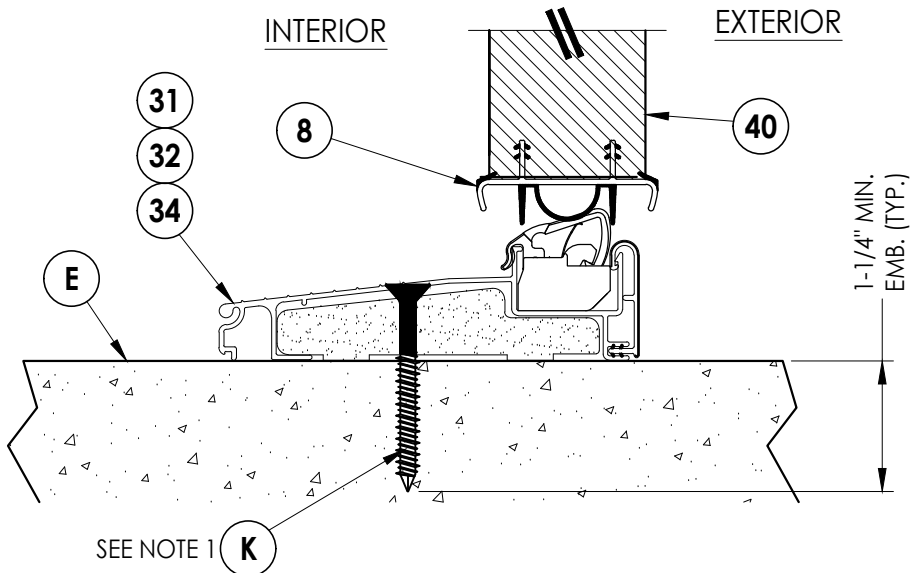
2 VERTICAL CROSS SECTION 8 Inswing configuration
