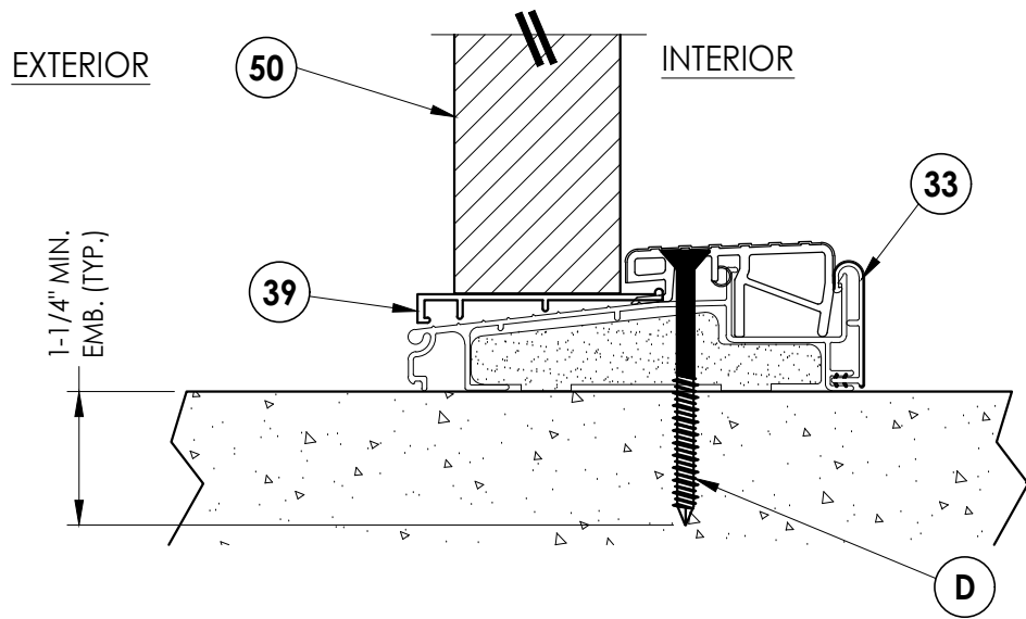
3 VERTICAL CROSS SECTION 8 Outswing configuration
