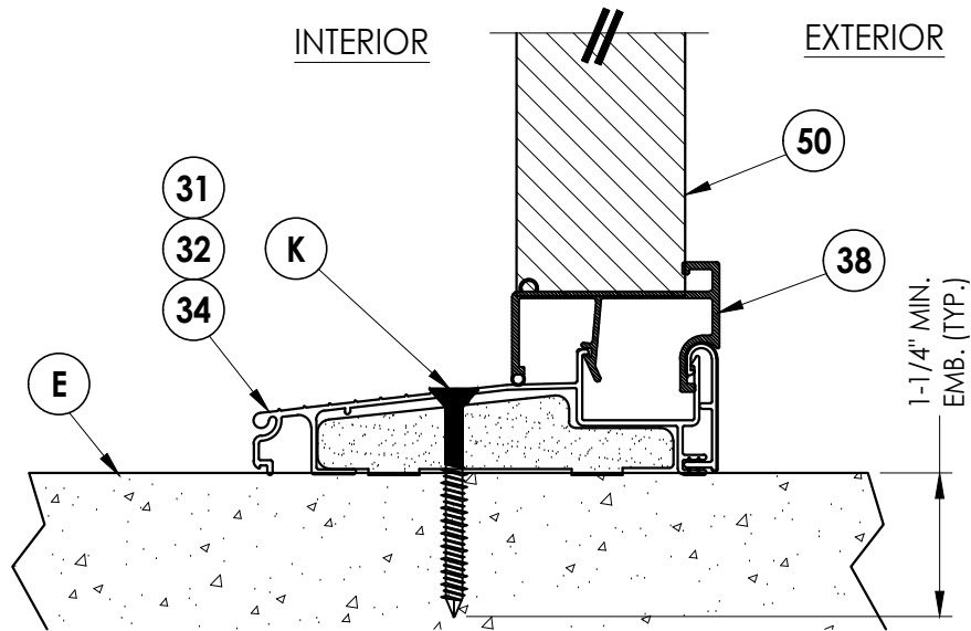
2 VERTICAL CROSS SECTION 8 Inswing configuration
